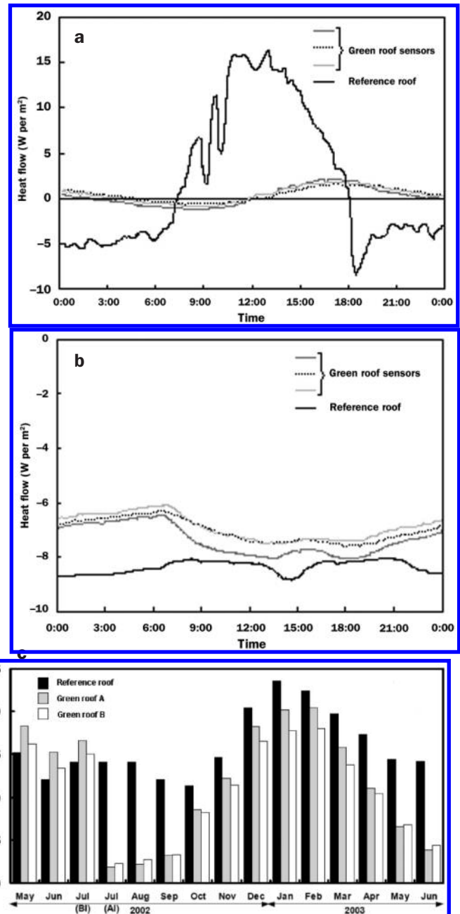
Figure 5. Heat flux across roof membranes for different roofing systems in Toronto, Ontario, Canada, on (a) a summer day (26 June 2003) and (b) a typical winter day with light snow coverage (23 January 2003), indicating that the green roof reduces the temperature fluctuations within the roofing system. Positive heat flux values indicate that net heat flux is from the outside into the building; negative values indicate that the net flux is from the inside to the outside. The green roof had 10 centimeters (cm) of light-colored growing medium. (c) Comparison of the average daily heat flow through the green roofs and reference (conventional) roof over two years. Green roofs were installed in late July 2002. Green roof A has 10 cm of light-colored growing medium; green roof B has 7.5 cm of dark-colored growing medium. Both were installed in Toronto. Abbreviations: AI, after installation; BI, before installation; kWh, kilowatt-hour; W, watt. Graphs are redrawn from Liu and Minor (2005).
